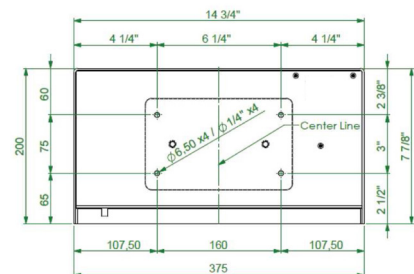
Installation from back
