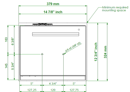
Installation from bottom
